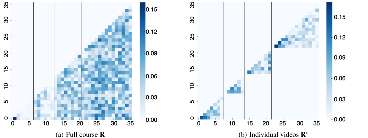
Figure 6: Visualizations of the prerequisite matrices extracted in two ways: (a) \mathbf{R} across the entire course, and (b) \mathbf{R}^v for each video v separately. The (s, s') th entry (the entry on the s th row and s' th column, with s < s' ) characterizes how much segment s serves as a prerequisite of segment s' . The solid lines delineate the four different videos.
