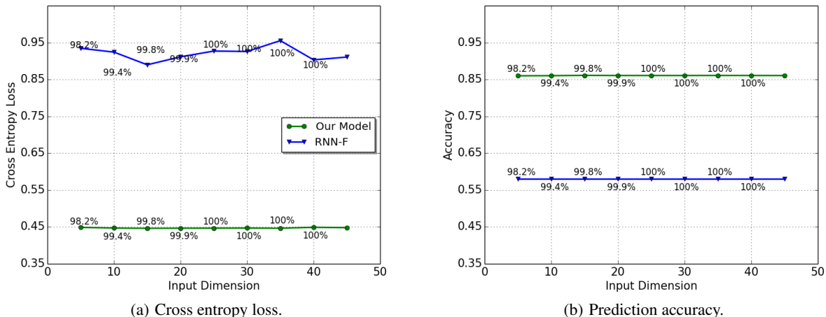
Figure 5: Prediction performance on the validation set as the dimension of the input word embedding ( D ) is varied for both our model and RNN-F. For each point, we label the percentage of variance in the input explained by the top- D principal components. The performance remains largely unchanged in each case, which is consistent with over 98% of the variance being explained by the top-5 principal components (i.e., D = 5 ).
